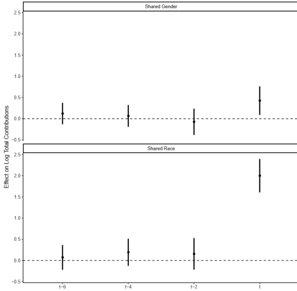
Figure A3: Granger-Style Causality Test
